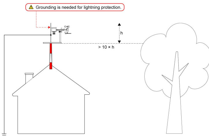
Figure 9 Grounding protection
