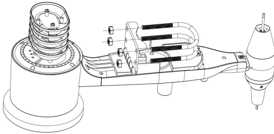
Figure 4 U-Bolt installation
